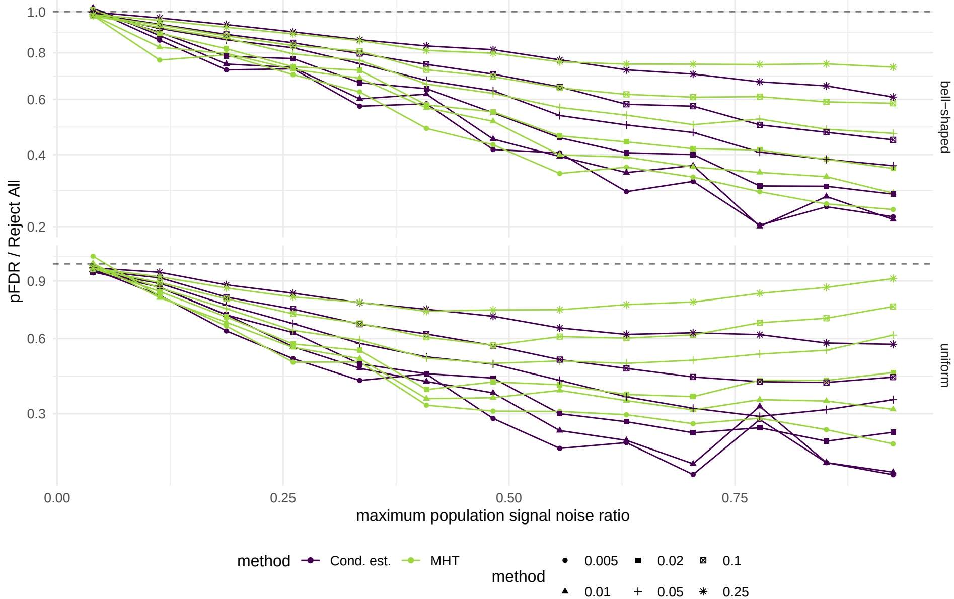
Positive False Discovery Rate of tests
