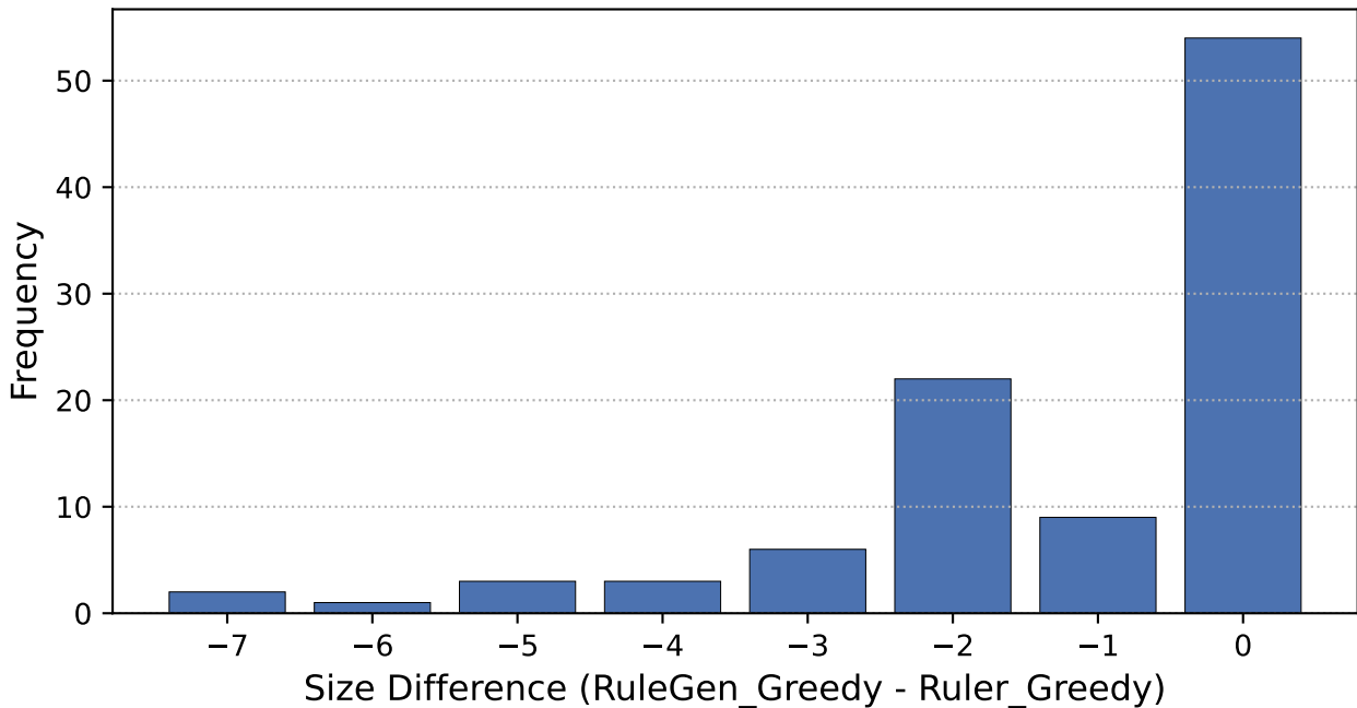
RuleGen_Greedy (0.680) Vs. Ruler_Greedy (0.366)
