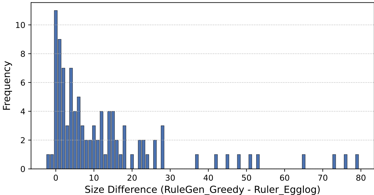
RuleGen_Greedy (14.018) Vs. Ruler_Egglog (3459.497)
