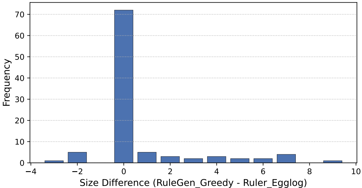
RuleGen_Greedy (0.698) Vs. Ruler_Egglog (121.322)
