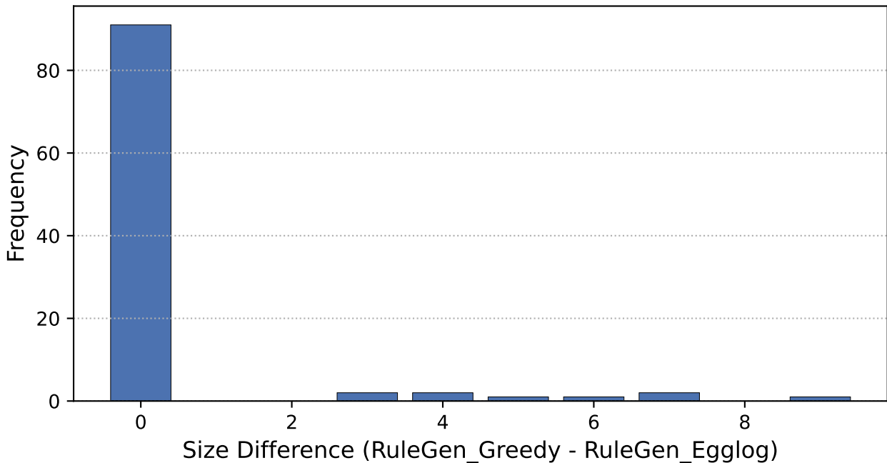
RuleGen_Greedy (0.699) Vs. RuleGen_Egglog (43.461)
