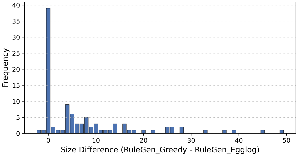
RuleGen_Greedy (14.179) Vs. RuleGen_Egglog (48.633)
