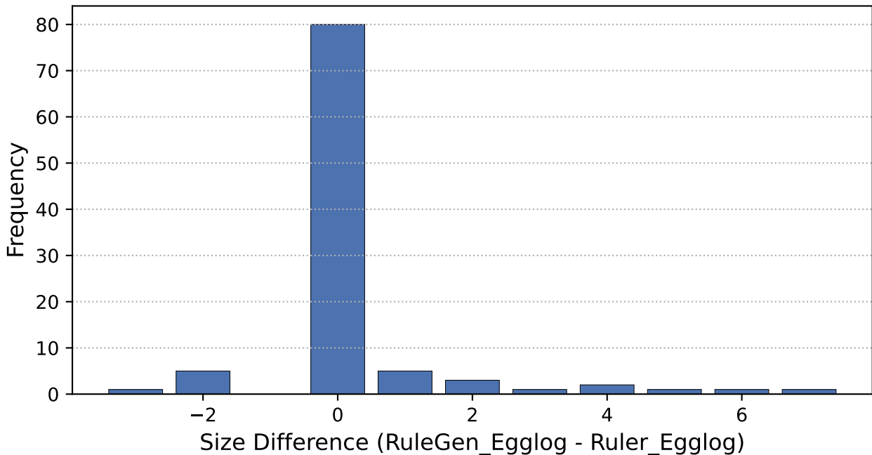
RuleGen_Egglog (44.064) Vs. Ruler_Egglog (118.449)
