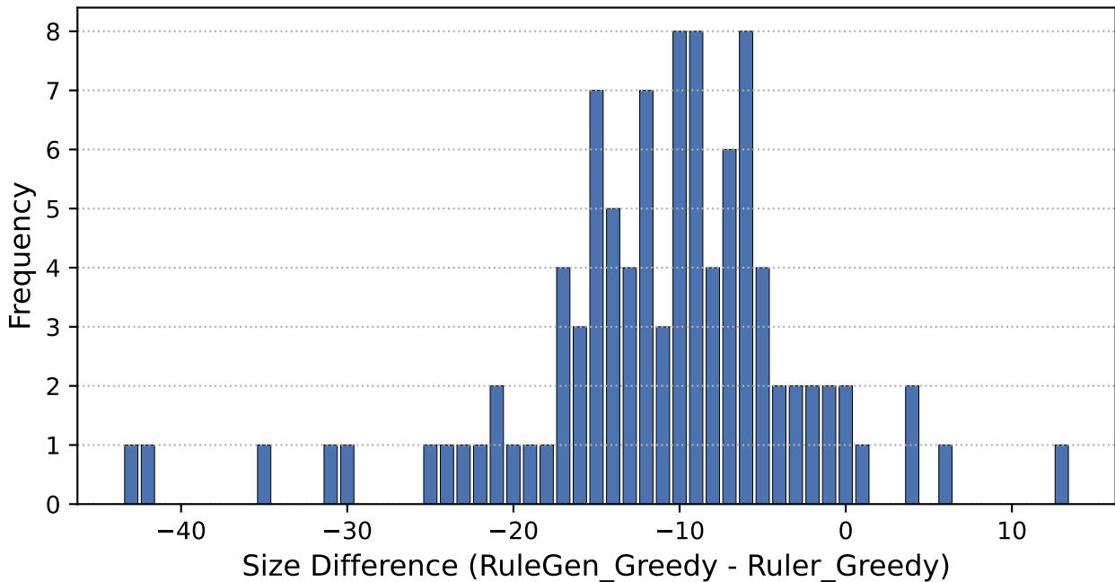
RuleGen_Greedy (14.412) Vs. Ruler_Greedy (13.707)
