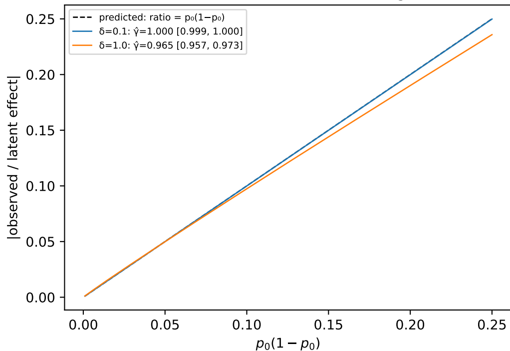
1.7 observed effect vs baseline (logit link)
