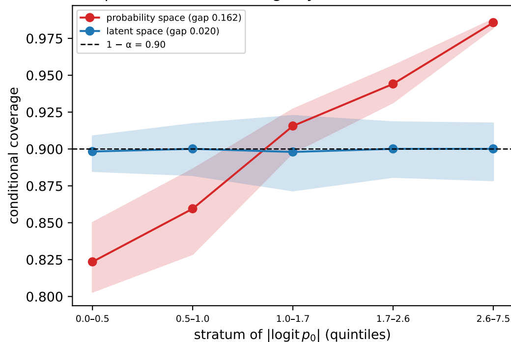
1.9 split-conformal coverage by baseline stratum ( \alpha=0.1 )
