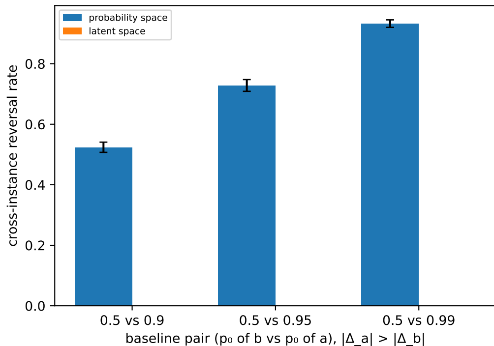
1.8 rank reversal rate
