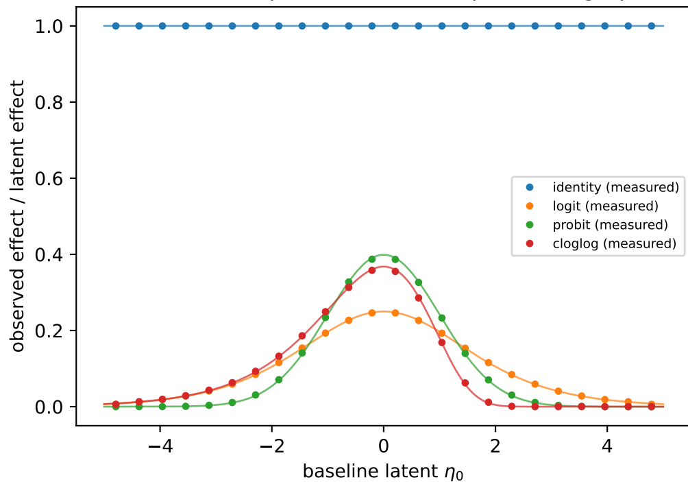
1.6 link sweep ( \delta=0.1 ); lines = predicted g'(\eta_0)
