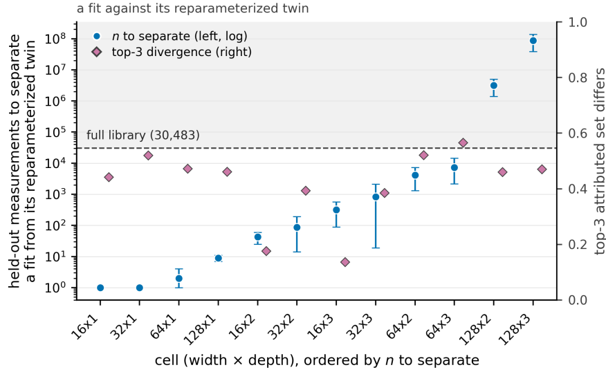
Figure 5: Separability and top-3 divergence for a fit against its own reparameterized twin, not for independently trained pairs. The requirement spans more than eight orders of magnitude here and two cells exceed the full library, where the main-text population separates with fewer than three measurements in every cell (Figure 3). Left axis logarithmic; the dashed line is the full library.
