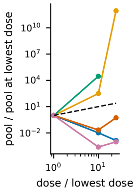
(a) thermodynamic K
