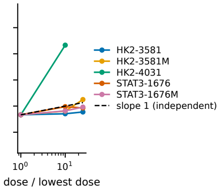
(b) site-class K
