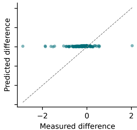
Chemistry GNN
