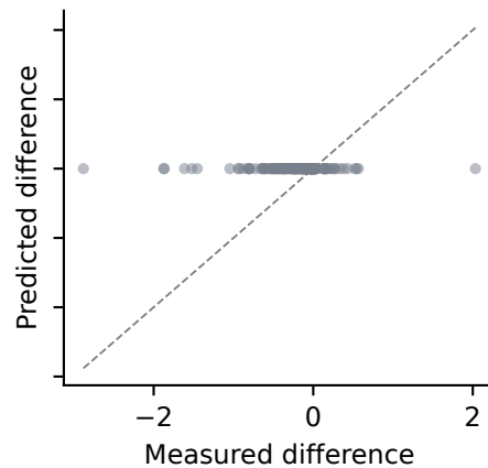
GNN without chemistry
