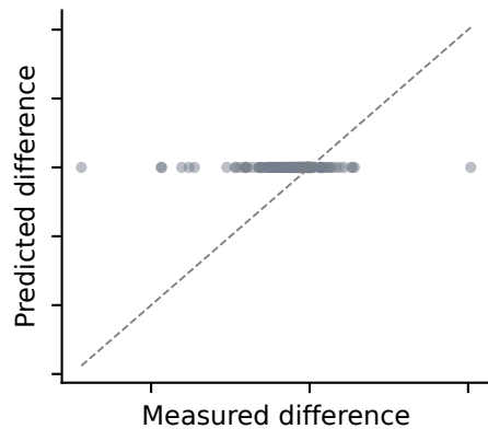
Chemistry GNN
