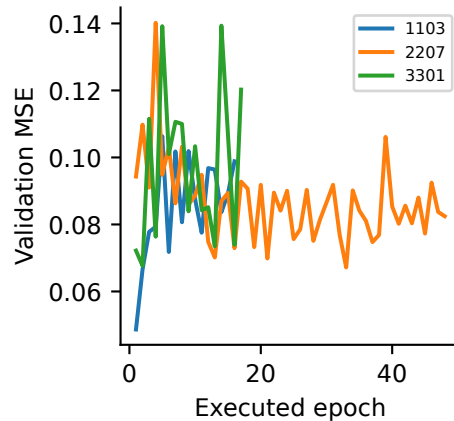
Chemistry GNN
