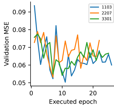
GNN without chemistry
