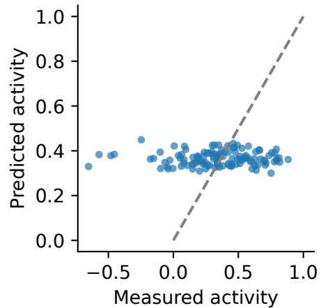
GNN
