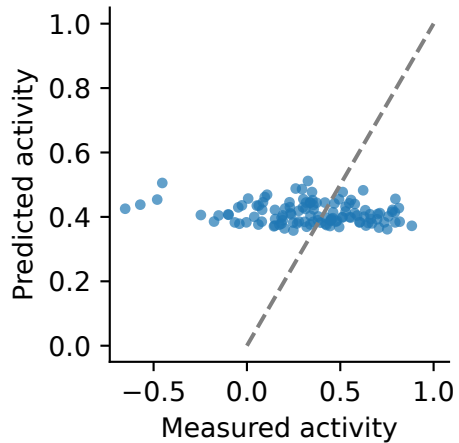
Chemistry tree
