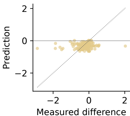
Pair tree
