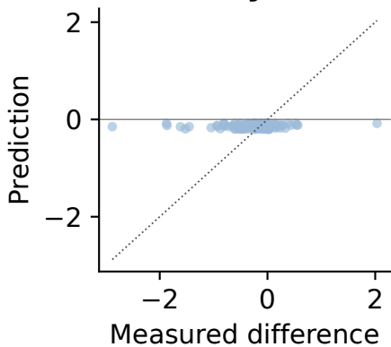
Activity GNN
