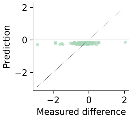
Pair GNN
