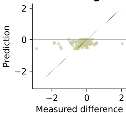
Pair ridge
