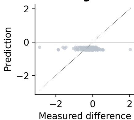
Training mean
