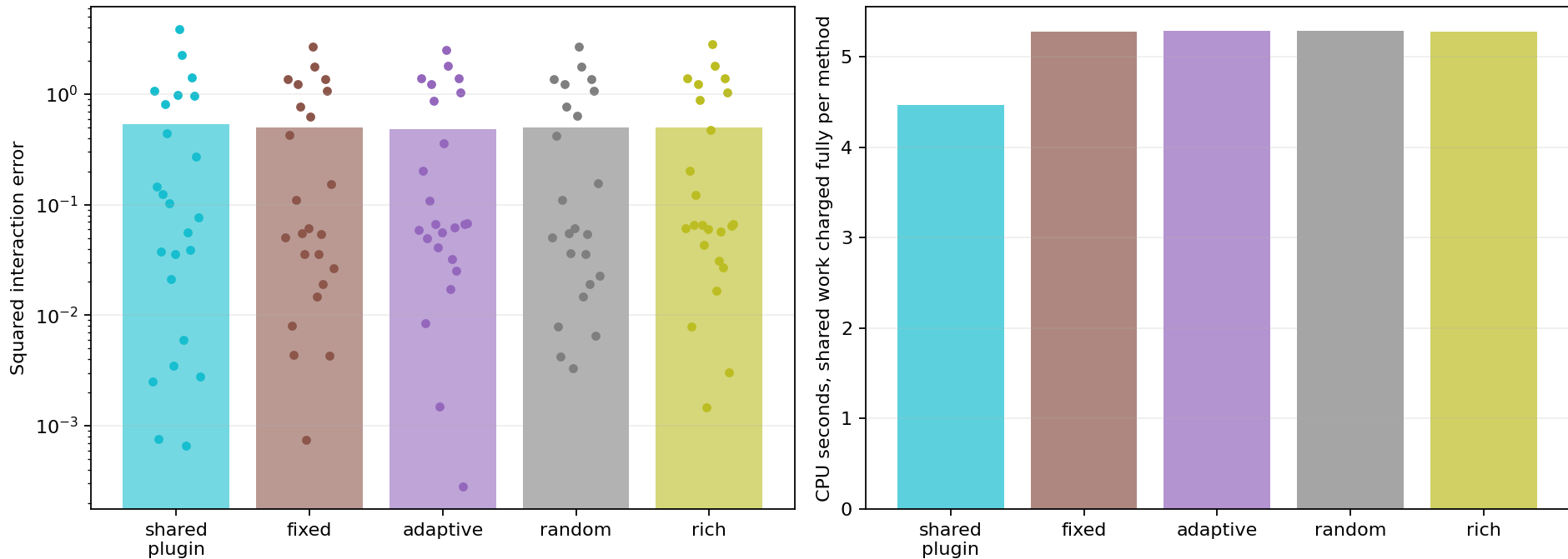
Mechanism ablation with the same nuisance fits
