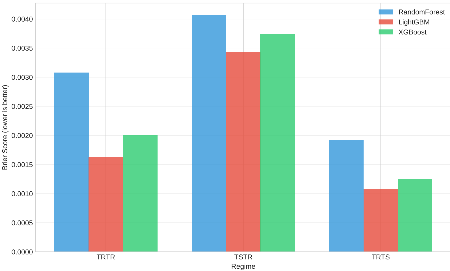
Calibration: Brier Score
