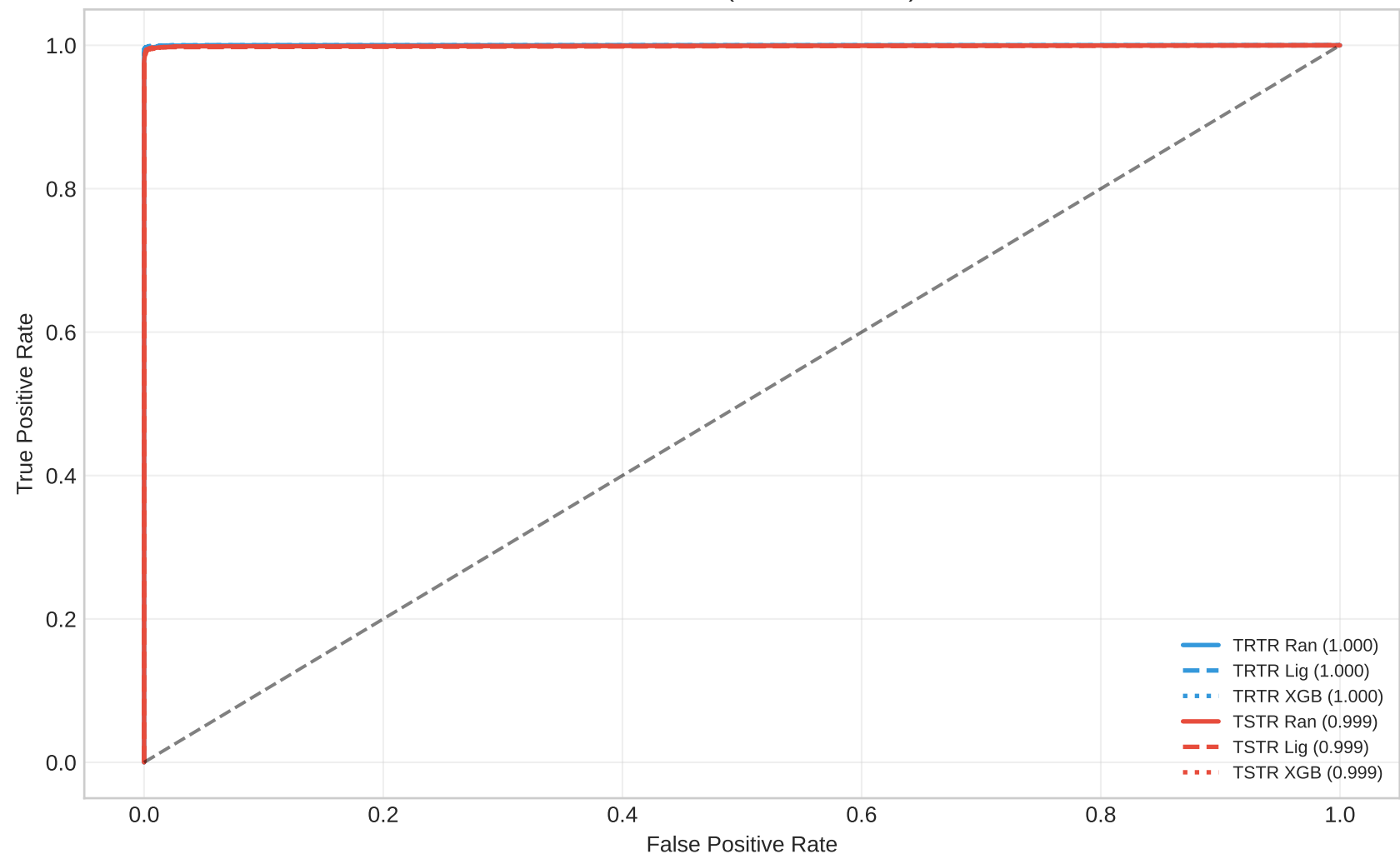
ROC Curves (Real Test Data)
