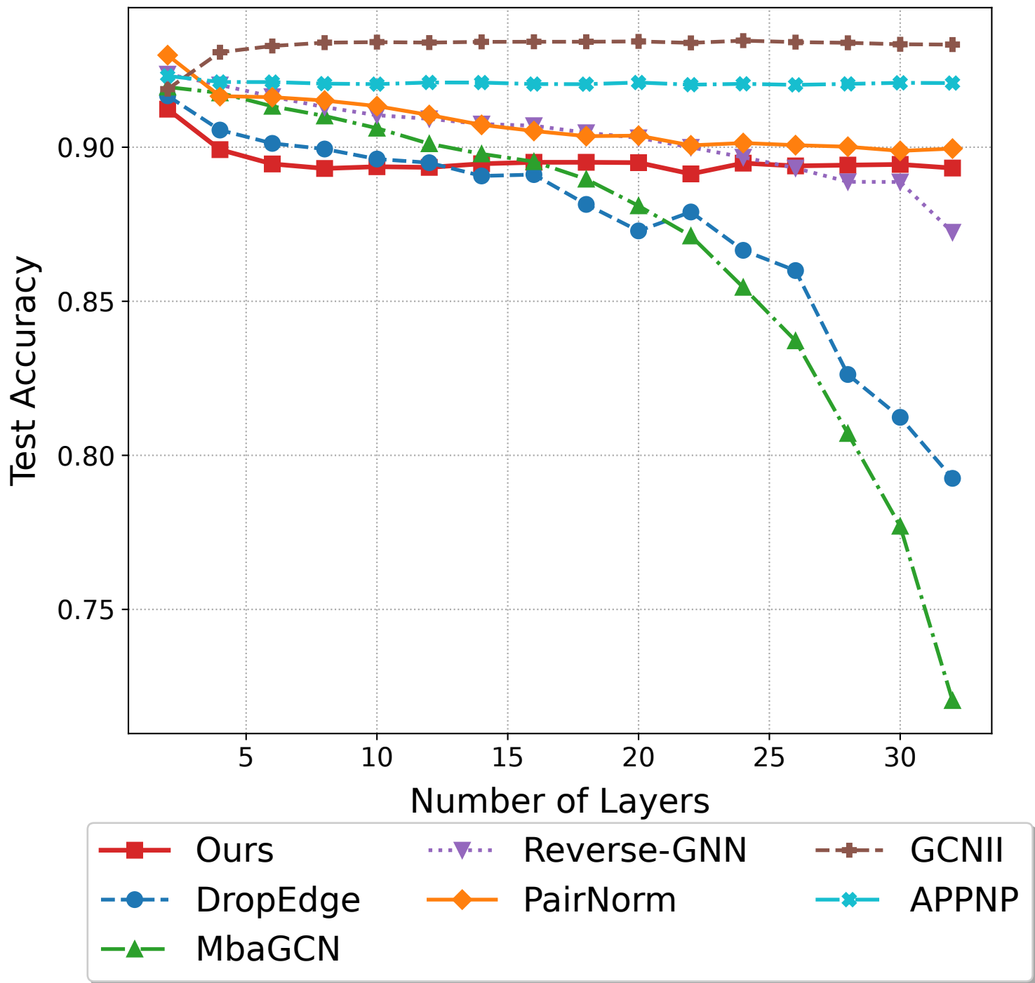
Balanced Two-Cluster Sampling on PubMed
