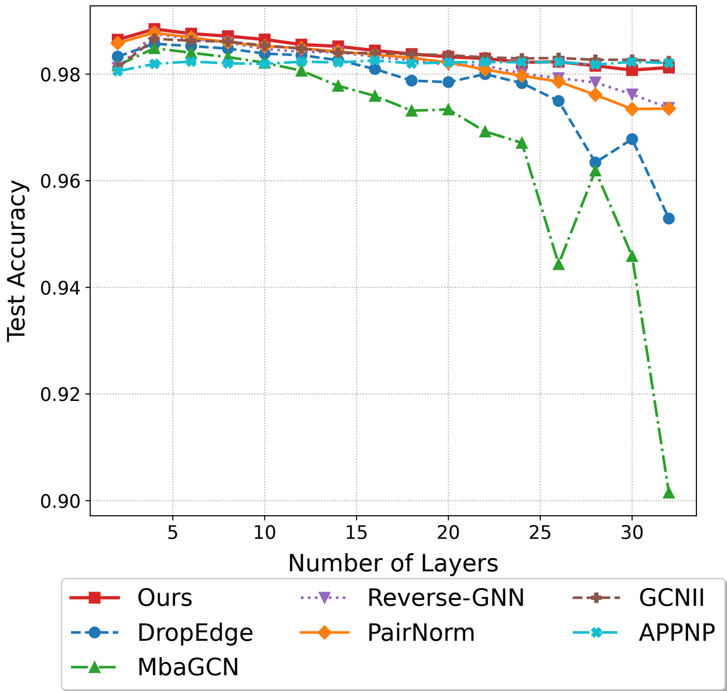
Balanced Two-Cluster Sampling on ogbn-products
