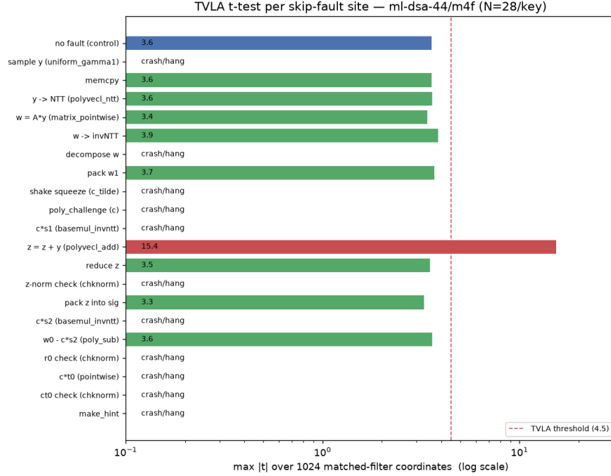
Figure 3: TVLA twin of the verdict: only the mask-removal site rises above the threshold.
