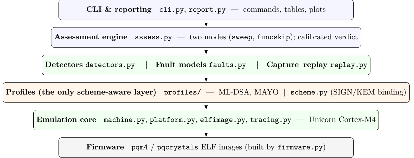
Figure 1: Layered architecture. Scheme-specific knowledge lives only in profiles/ and scheme.py ; every other layer works on instructions, memory, and feature matrices.
