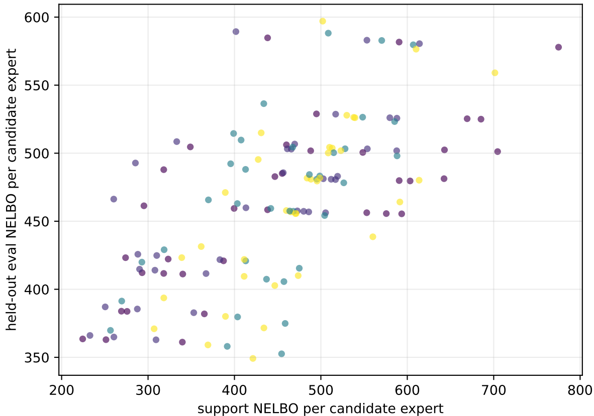
Direct support-NELBO: heldout center 1
