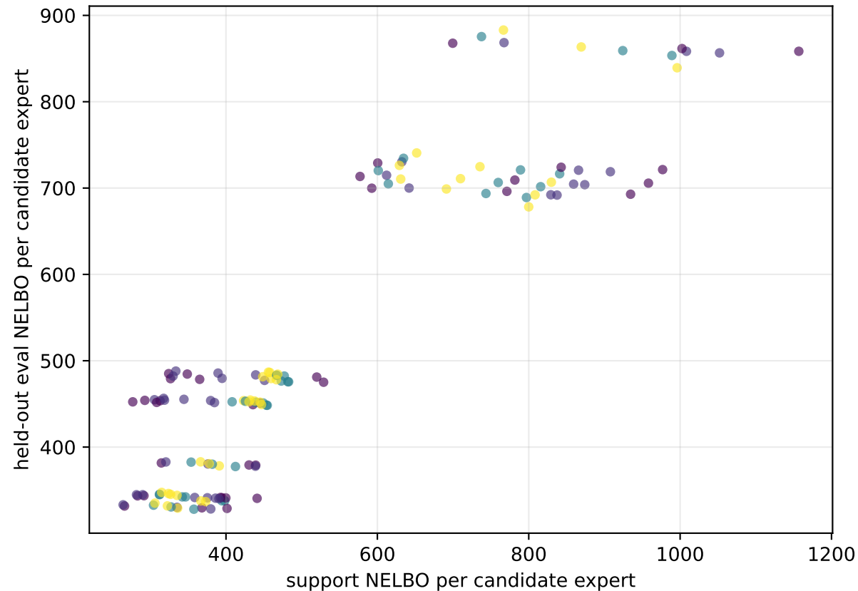
Direct support-NELBO: heldout center 2
