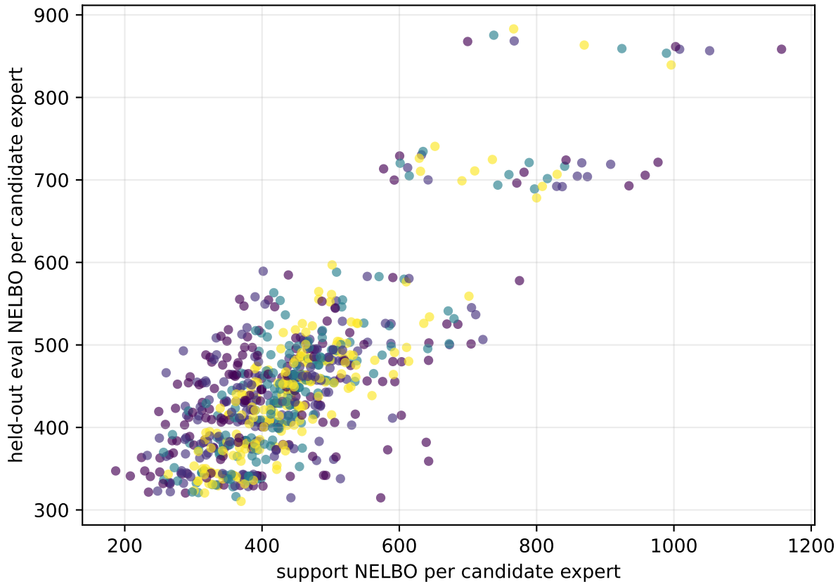
Direct support-NELBO: pooled candidates
