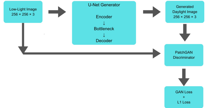
Fig. 4: Architecture of the proposed Pix2Pix model.
