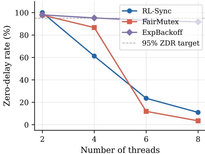
(b) ZDR vs Concurrency
