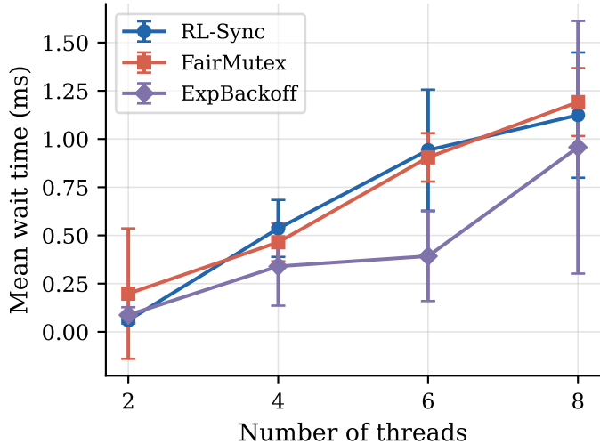
(a) Wait Time vs Concurrency
