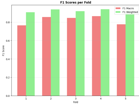
Figure 1: F1 scores of model 2
