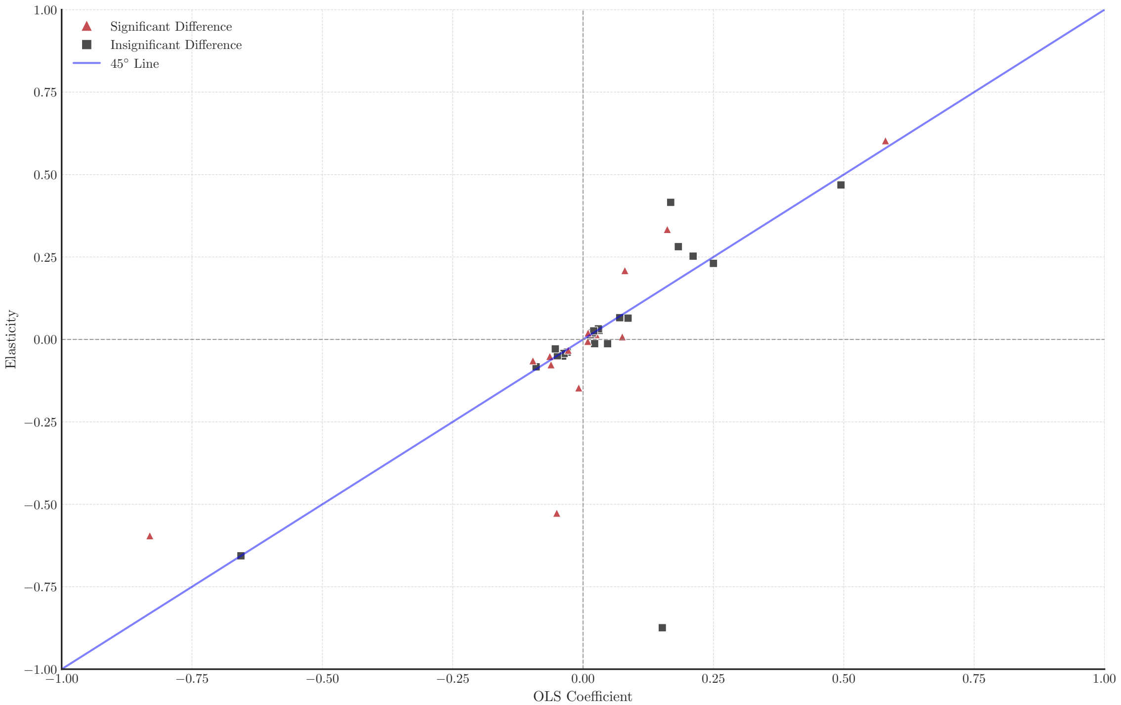
DR Elasticity vs OLS Coefficient
