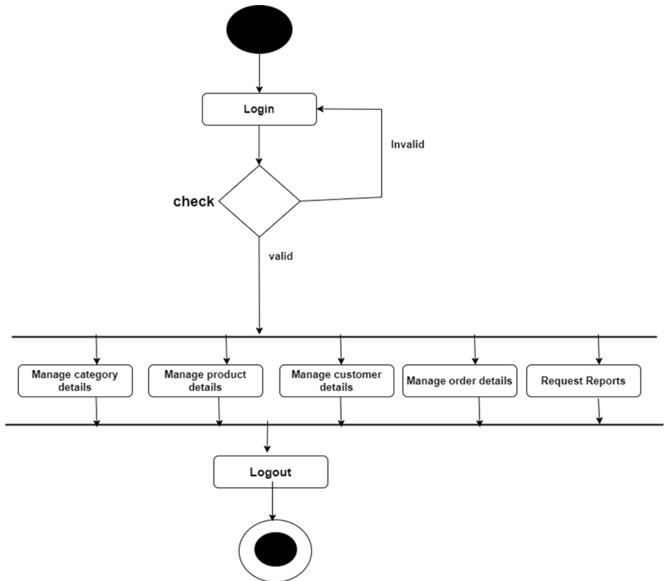
Figure 7 : Activity diagram of admin
