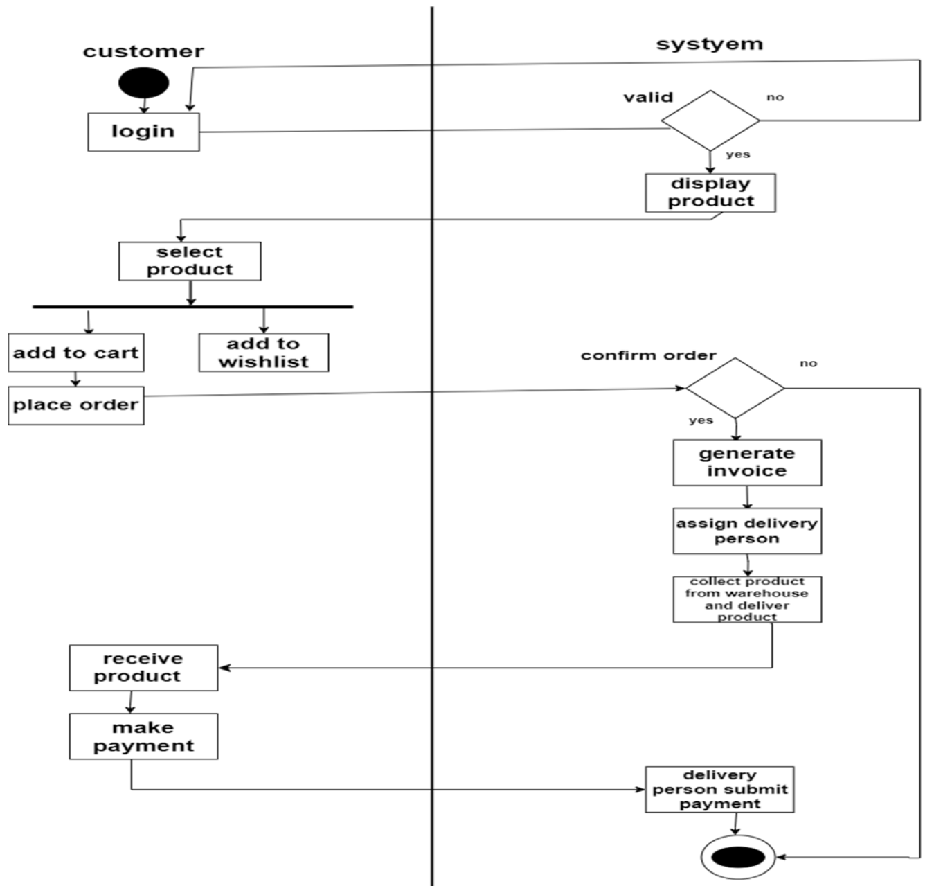
Figure 8 : Activity Diagram of User(customer , system)
