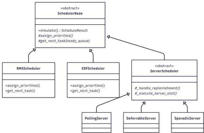
Class Hierarchy
