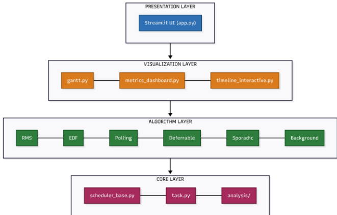
Layered Architecture
