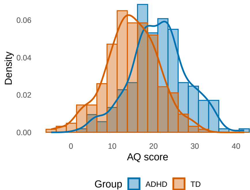
A AQ Distribution by Group
