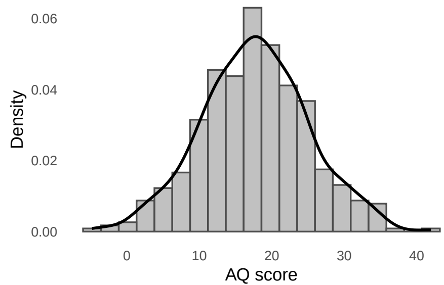
B AQ Distribution: Overall
