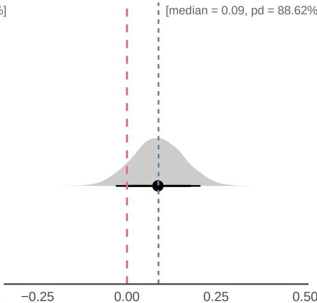
sigma_rho
