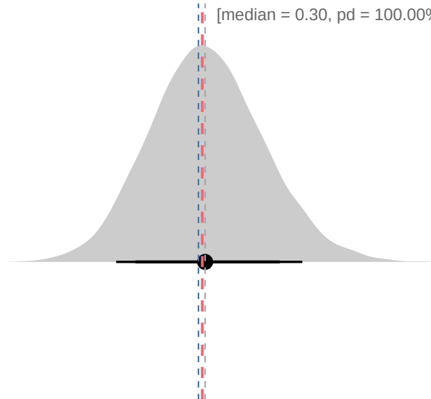
sigma_log_beta
