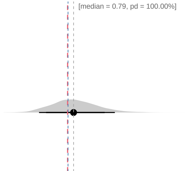
sigma_gamma
