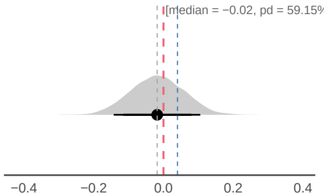
sigma_gamma
