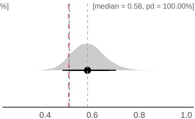
sigma_gamma
