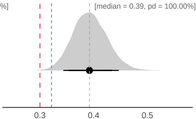
mu_logit_gamma
