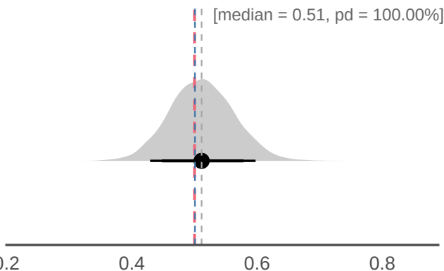
sigma_rho
