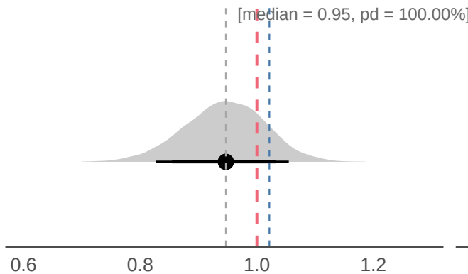
sigma_rho
