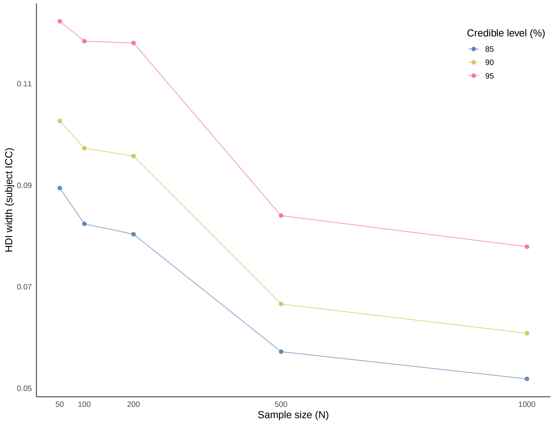
CBCU utilities: subject-ICC HDI width by sample size
