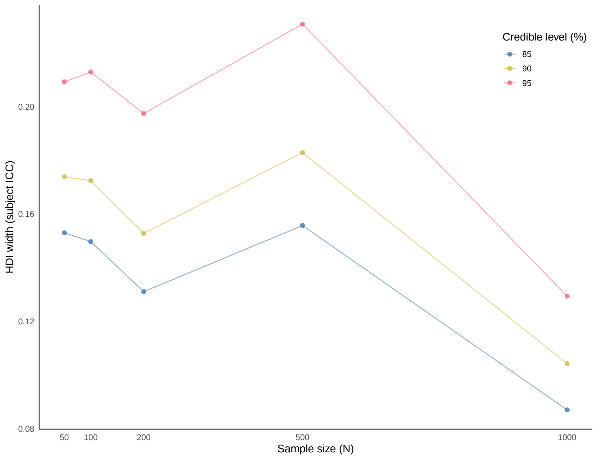
PHQ9 items: subject-ICC HDI width by sample size
