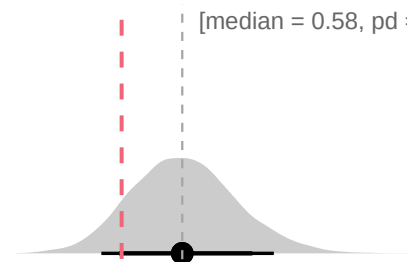
sigma_gamma
