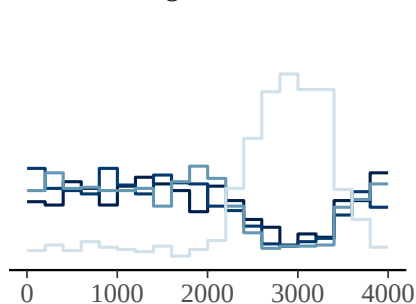
sigma_rho
