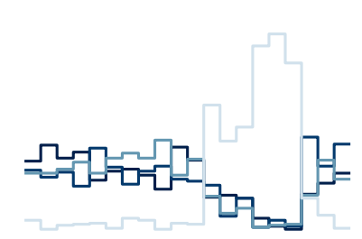
mu_logit_key_decay
