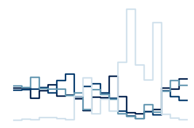
sigma_log_beta
