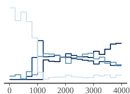
sigma_key_decay
