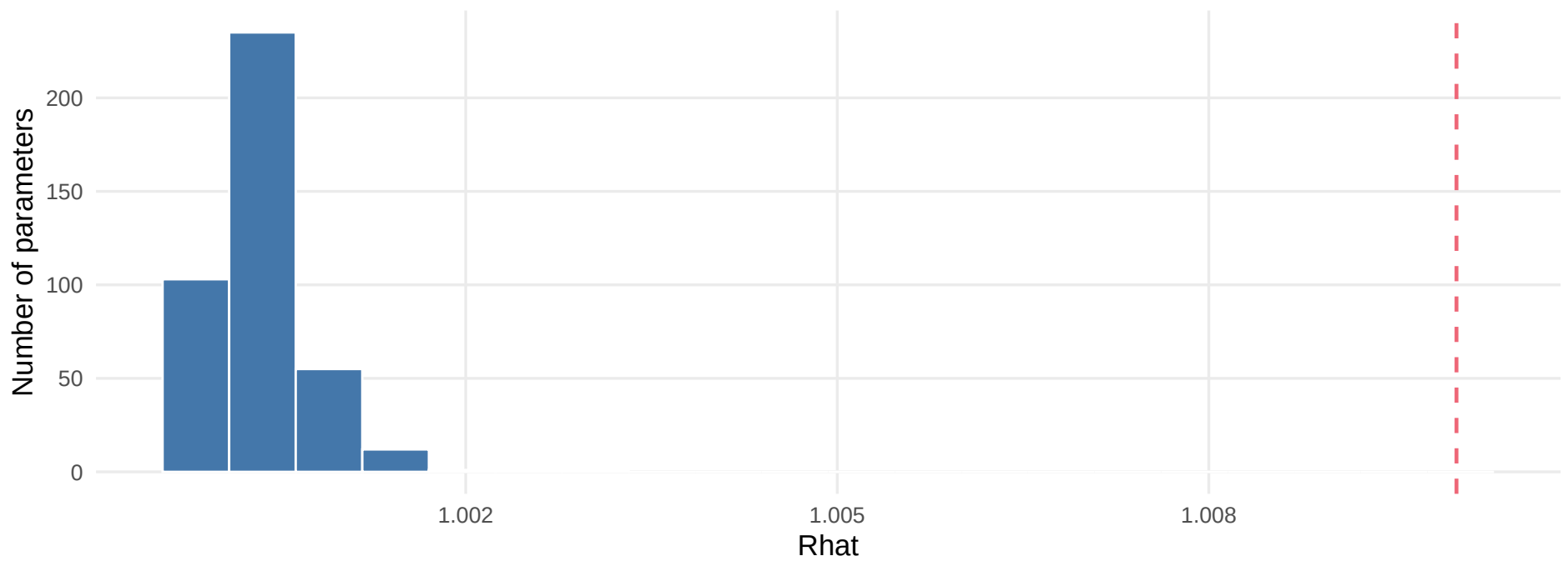
Rhat (dashed line = 1.01)
