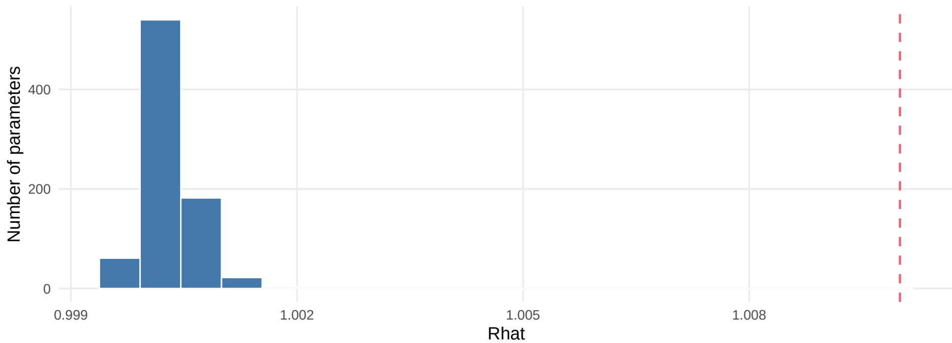
Rhat (dashed line = 1.01)
