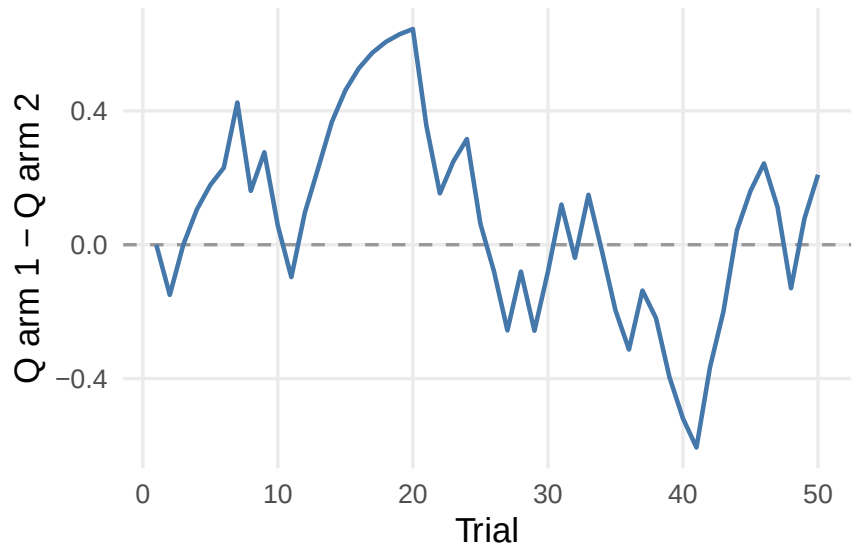
Delta Q
