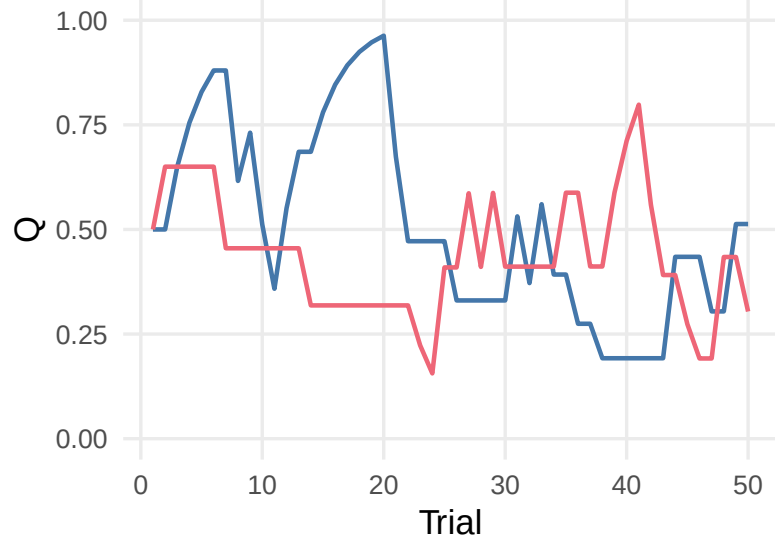
Delta Q
