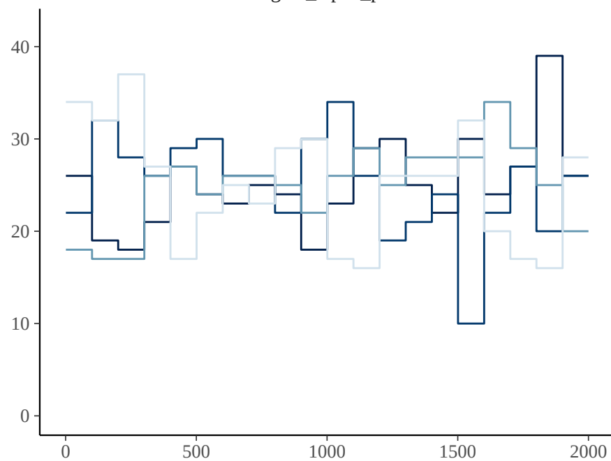
sigma_alpha_per
