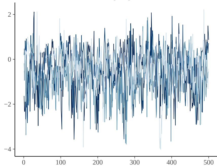
mu_alpha_per
