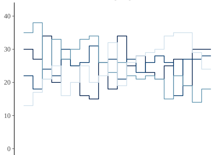
mu_alpha_per
