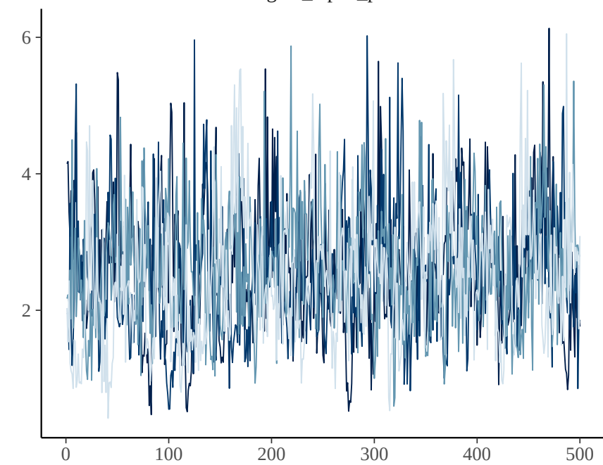
sigma_alpha_per
