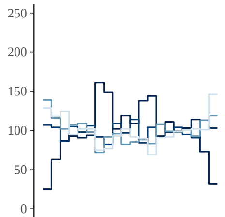
b_Intercept
