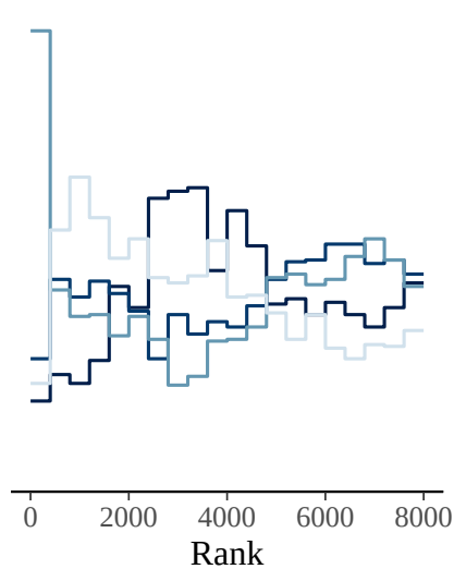
sigma
