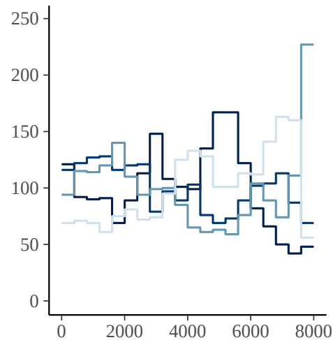
d_subject_id:session_id__Intercept
