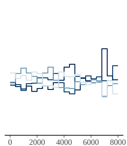
sd_subject_id__Intercept
