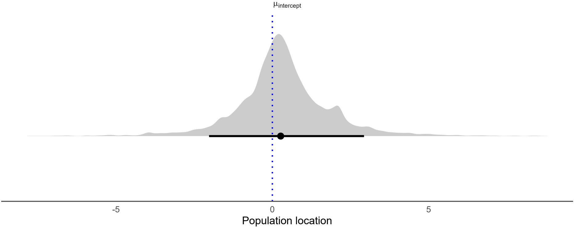
Figure 1. Posterior density of the population location (intercept). The dotted blue line marks the true generating value.
