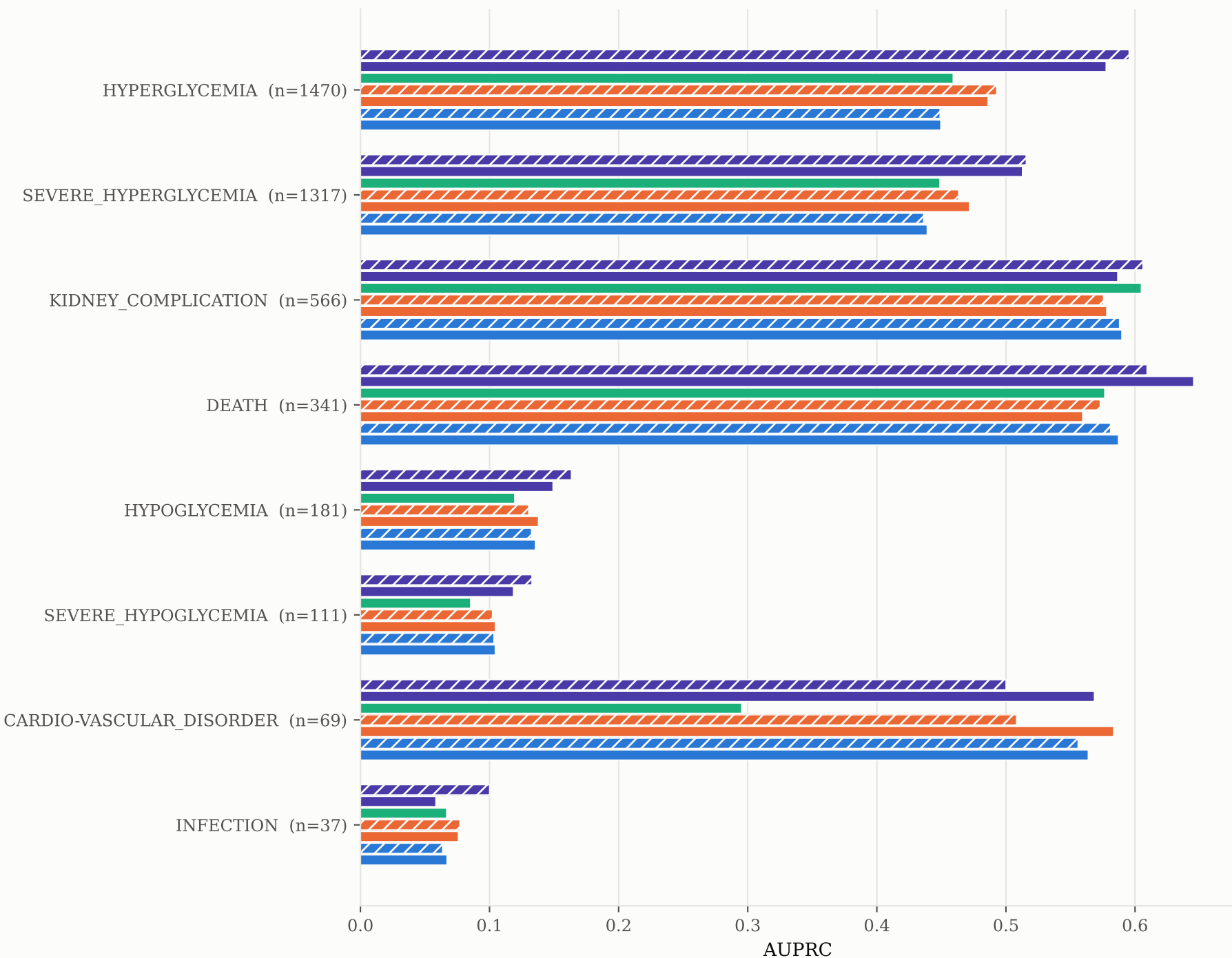
Per-target AUPRC at K=4
