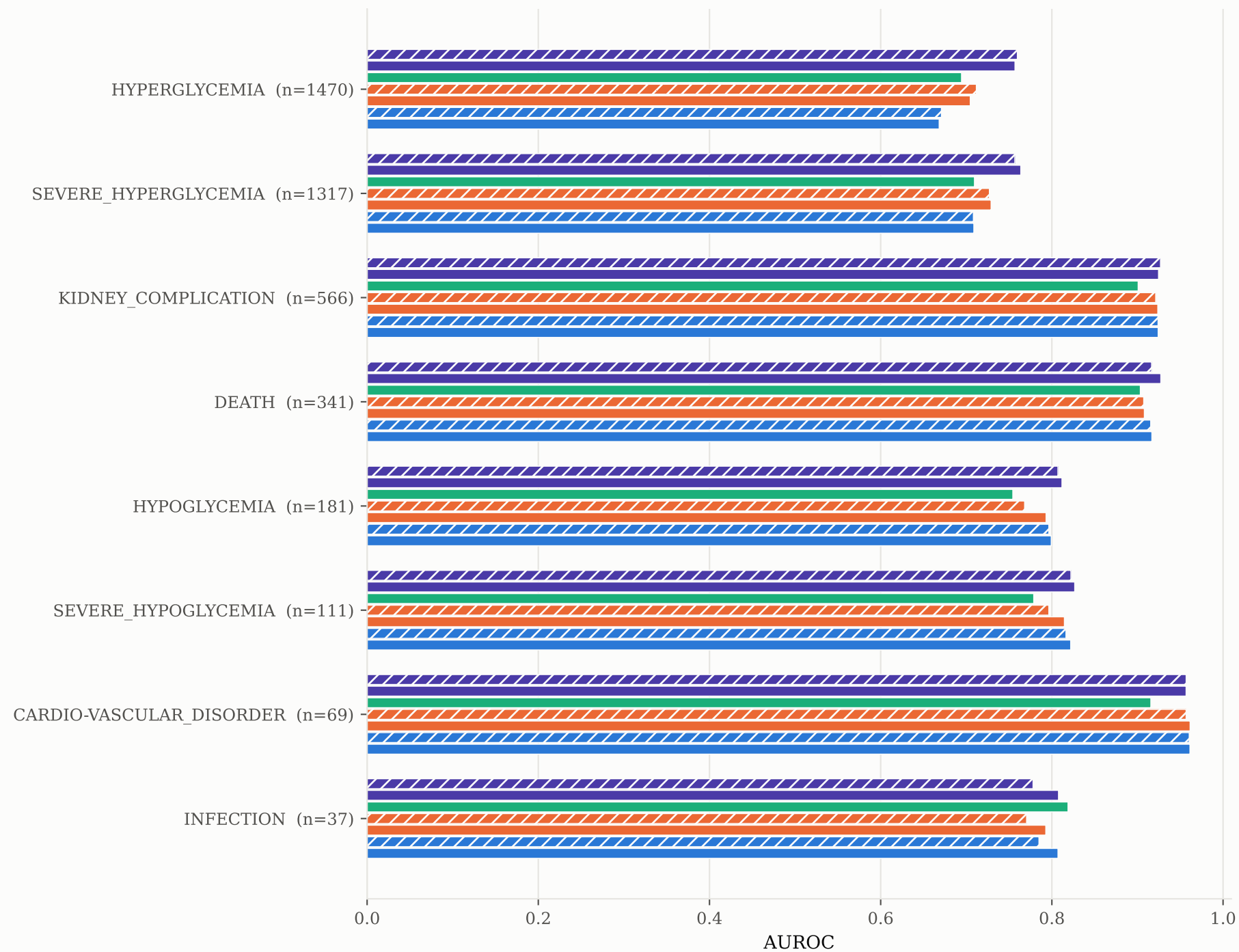
Per-target AUROC at K=4
