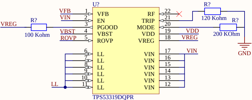
Buck Reguator IC
