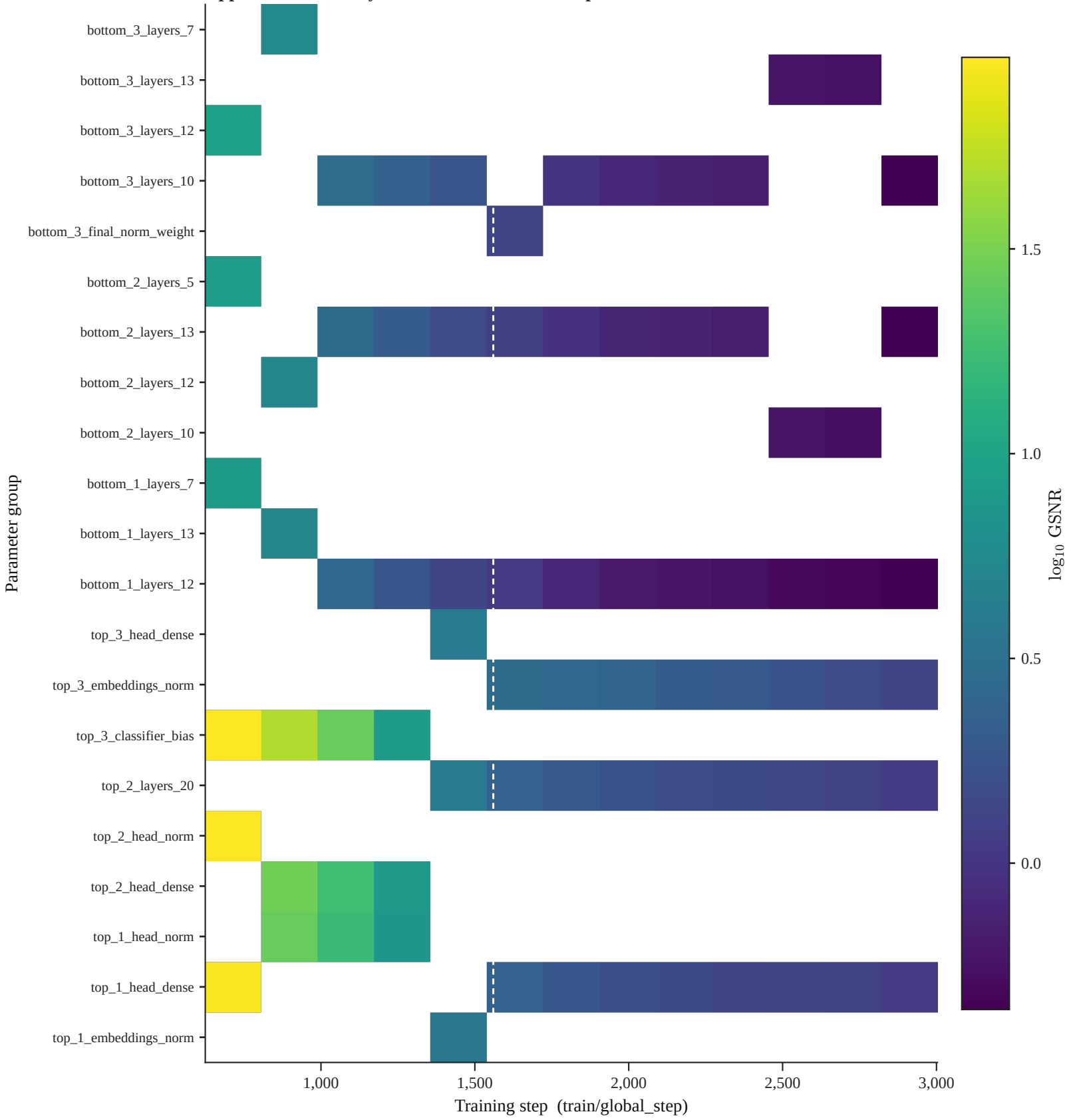
Appendix A2 — Layer-resolved GSNR heatmap
