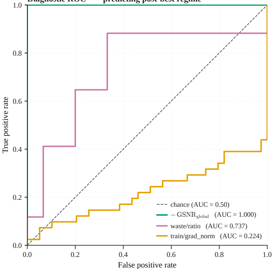
Diagnostic ROC — predicting post-best regime
