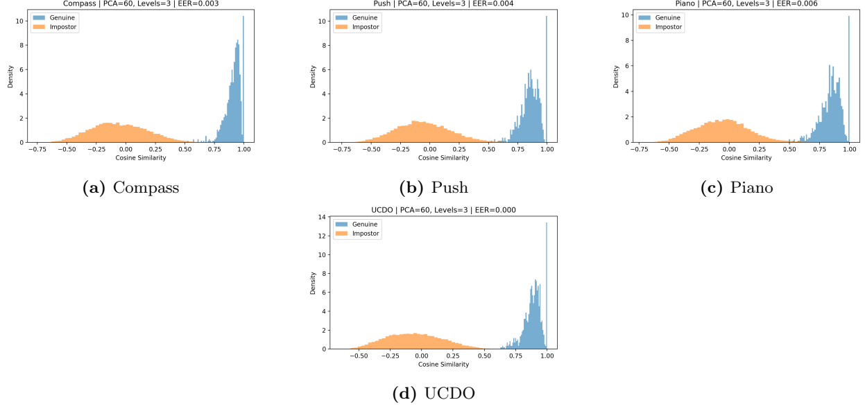
Figure 14: Cosine similarity plots for different Gestures for PCA+LDA solution
