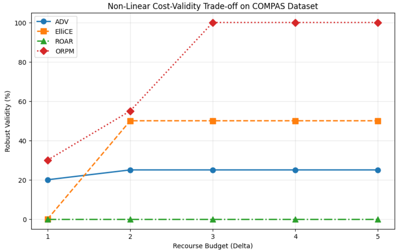
Figure 2: The cost validity trade-off for ORPM and baselines.
