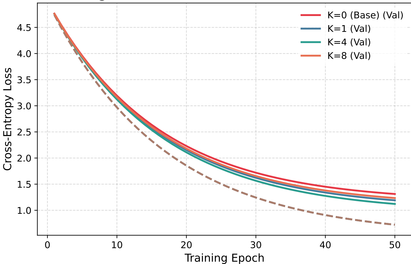
Training (Dashed) vs. Validation (Solid) Loss Curves
