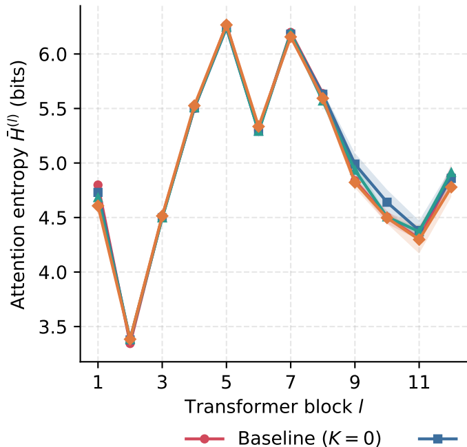
Absolute entropy
