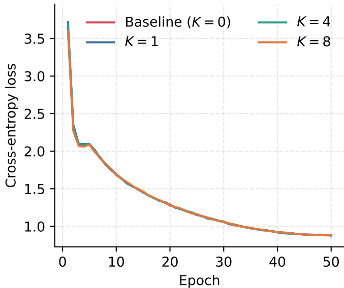
Training loss
