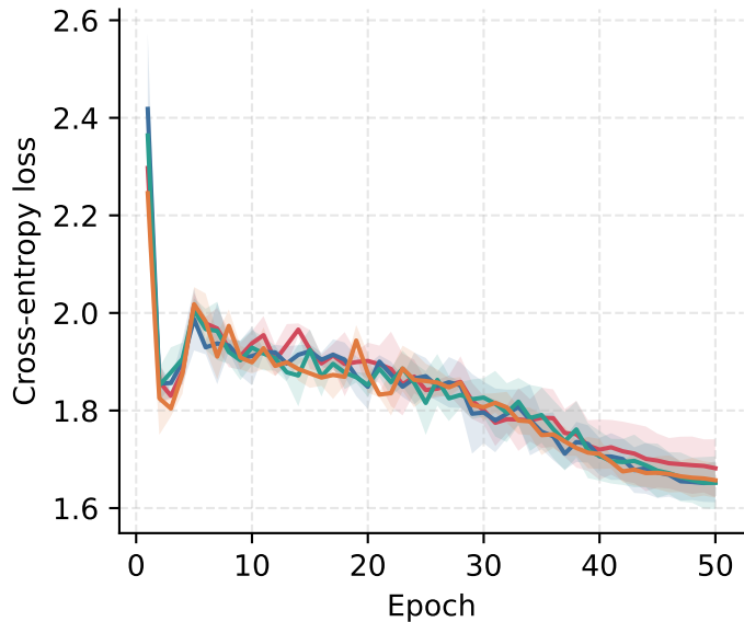
Validation loss
