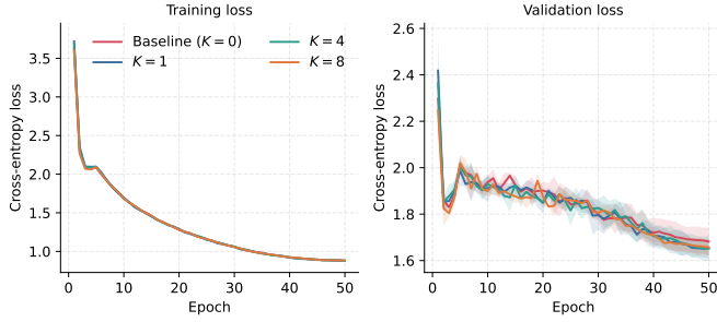
Fig. 4. Seed-averaged loss trajectories, \pm 1\sigma bands. Training curves are superimposed across arms; validation curves are dominated by the noise of a 1,000-image split.
