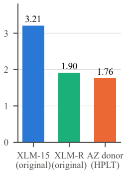
(a) Segmentation cost
