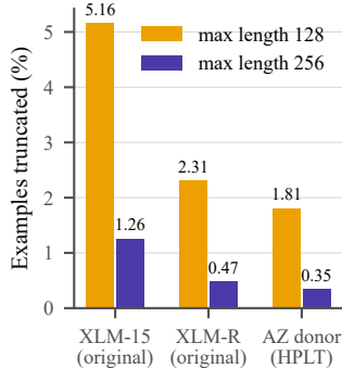
(c) Truncation, 27,914 examples
