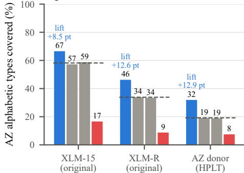
(b) Vocabulary overlap with Azerbaijani
