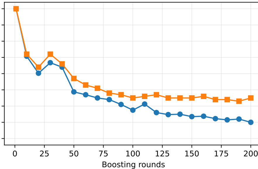
Digits High-Dimensional
