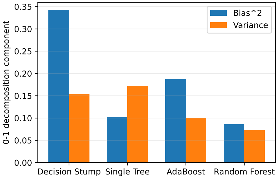
Bias-variance on balanced binary data
