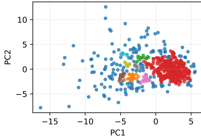
DBSCAN
